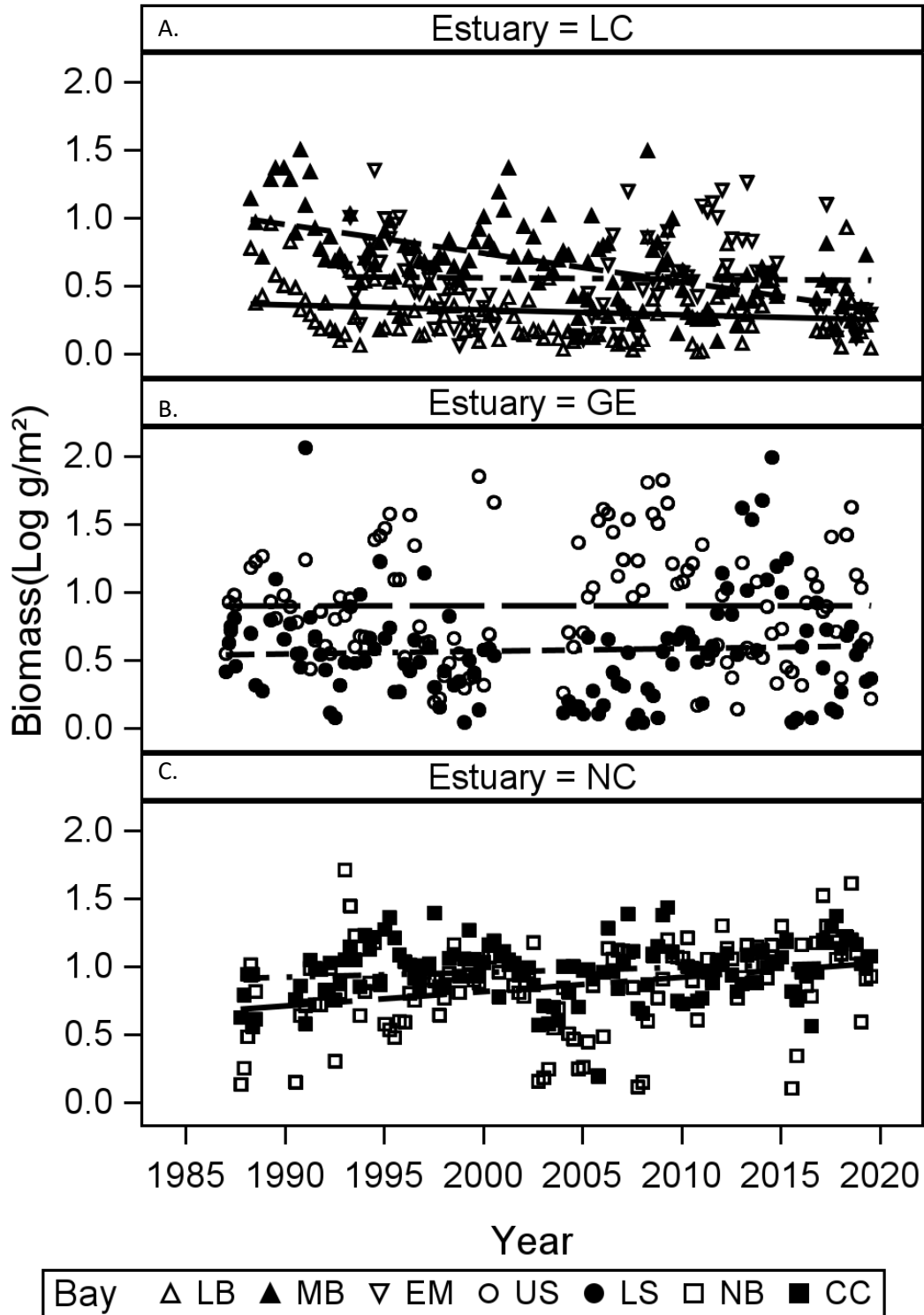
Figure 13. Average quarterly (January, April, July, and October) log 10 transformed benthic infauna biomass by bay from 1987-2018. Abbreviations and symbols defined in Figure 12. A) Lavaca-Colorado Estuary. B) Guadalupe Estuary. C) Nueces Estuary.
